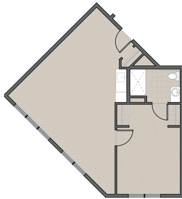
ONE BEDROOM SUITE FLOOR PLAN 778 SQ. FT.
